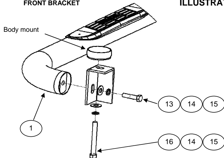
FRONT BRACKET
