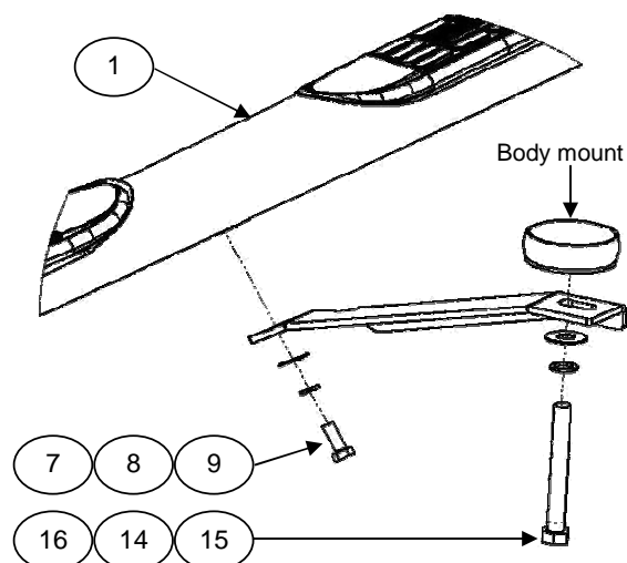
MIDDLE BRACKET
